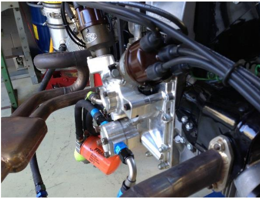
Dual Distributors
